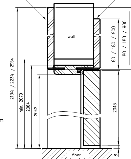
A-A Vertical cross-section side B side A
