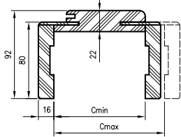
OR/ORC cross-section with T80 architrave
