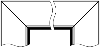
ORB connection at 45
