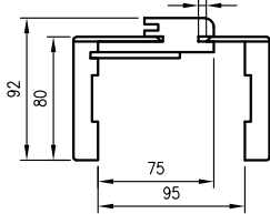
ORB horizontal cross-section
