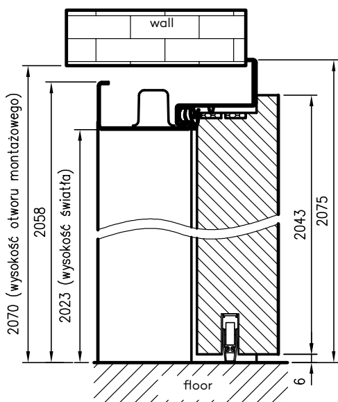
OLIMP EI-60 door leaf vertical cross-section
