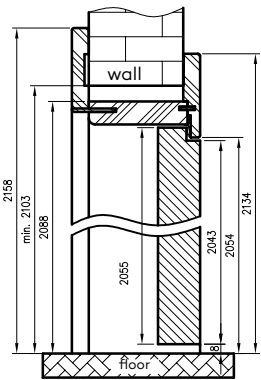
vertical cross-section of ORO
