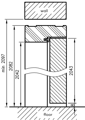
OPB vertical cross-section
