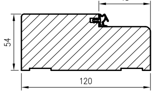
Cross-section of the wooden door frame for OLIMP EI60 doors
