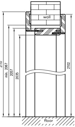
Vertical section of the adjustable tunnel with T63 architrave
