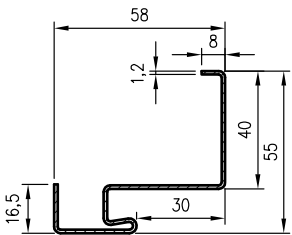
small angular steel door frame profile
