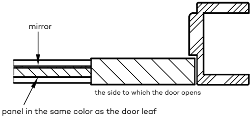
ESTRA 10 doors, non-rebated or rebated, in the "Reverse" variant
