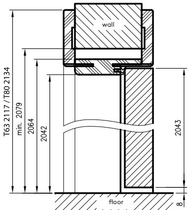
Vertical section of non-rebated door leaf
